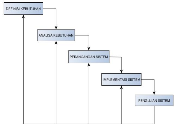
Gambar 1. Metode SDLC
