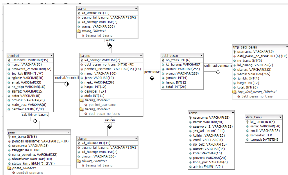
Gambar 5. ERD (Entity Relationship Diagram)
