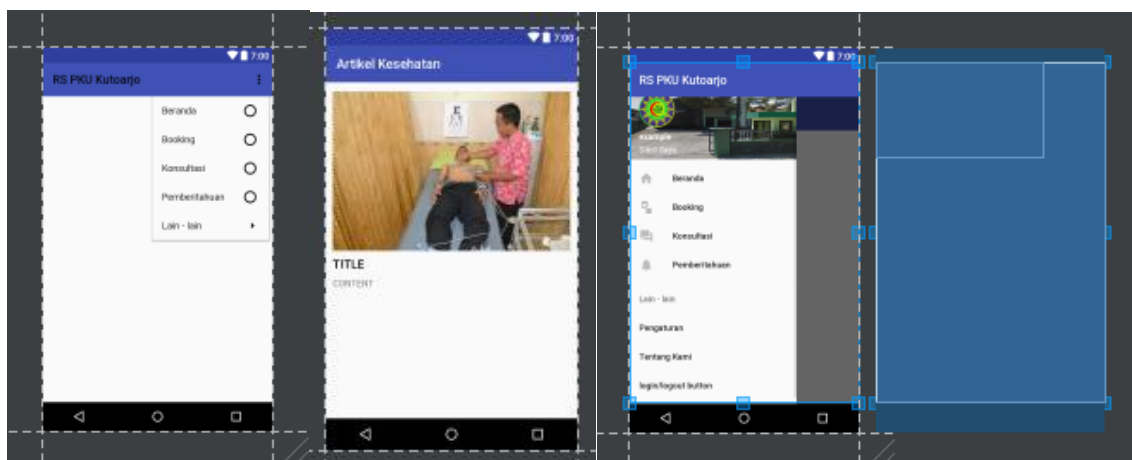
Figure 4. Interface Design
