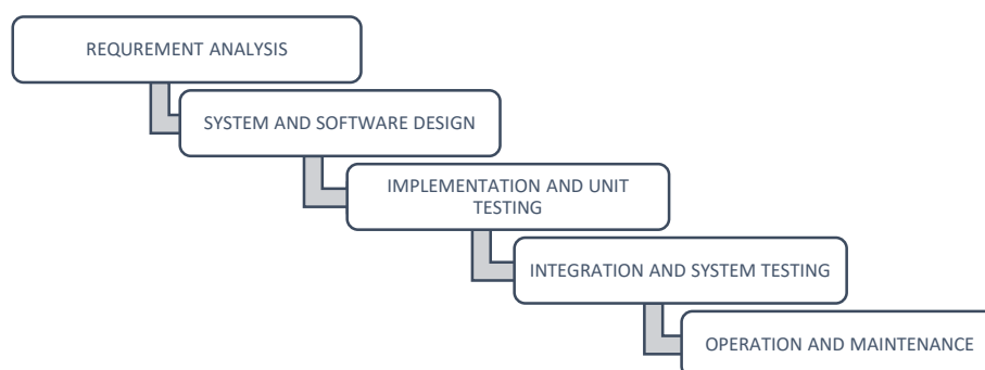
Figure 1. Waterfall model
