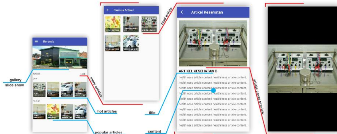
Figure 10. Home Interface
