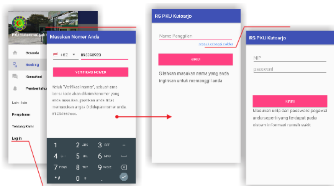
Figure 9. Login Interface
